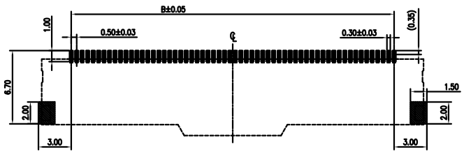
RECOMMENDED PCB PATTERN DIM. TOLERANCE : ±0.05
