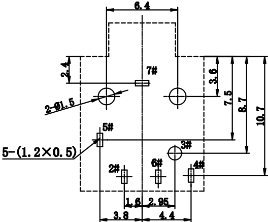
PCB Holes diagram Top View
