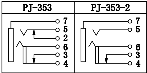
SCHEMATIC
