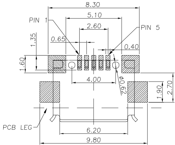
RECOMMENDED P.C.B. LAYOUT TOP VIEW (TOLRANCE: ±0.05)
