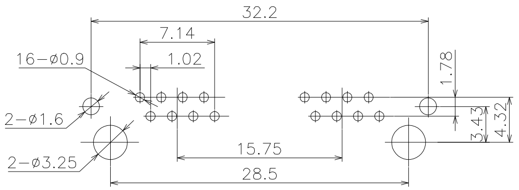
PCB LAYOUT (TOP VIEW) RECOMMENDED
