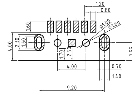
RECOMMENDED P. C. B LAYOUT TOP VIEW (TOLRANCE: \pm 0.05 )
