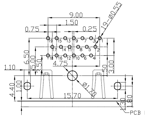
RECOMMENDED PCB LAYOUT (TOP VIEW) TOLERANCE FOR PCB LAYOUT IS ±0.05
