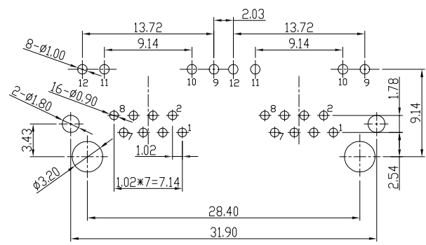
Recommend PCB Layout (Jack Top View) TOLERANCES:±0.05
